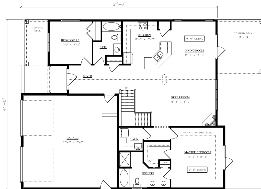
MAIN FLOOR PLAN 1492 SQ. FT.
