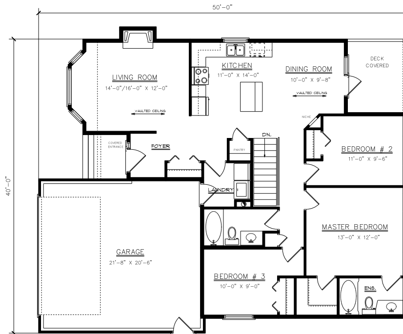
FLOOR PLAN 1270 SQ. FT.
