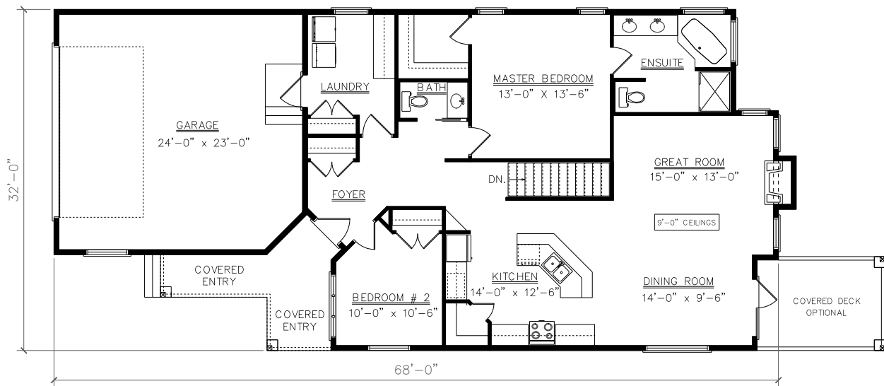
FLOOR PLAN 1342 SQ. FT.
