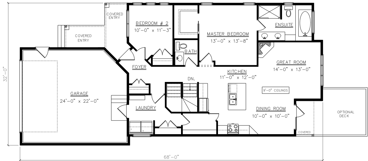
FLOOR PLAN 1260 SQ. FT.
