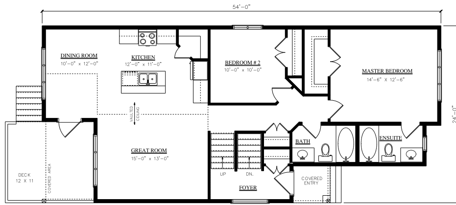
MAIN FLOOR PLAN 1108 SQ. FT.
