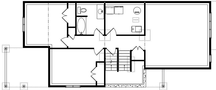
FOUNDATION PLAN
