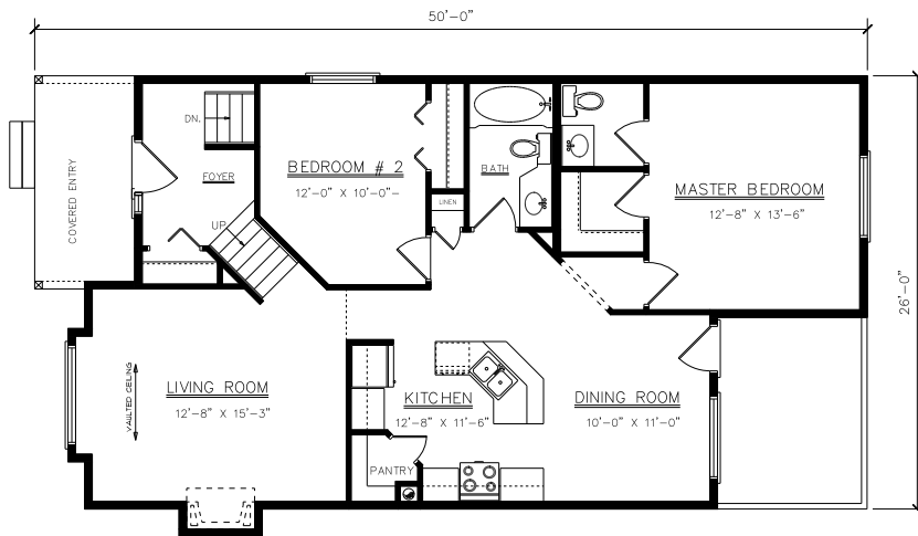
FLOOR PLAN
