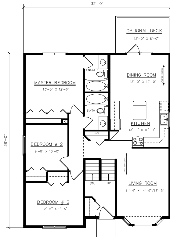
FLOOR PLAN 1190 SQ. FT.
