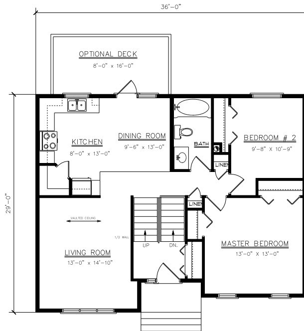
FLOOR PLAN 984 SQ. FT.
