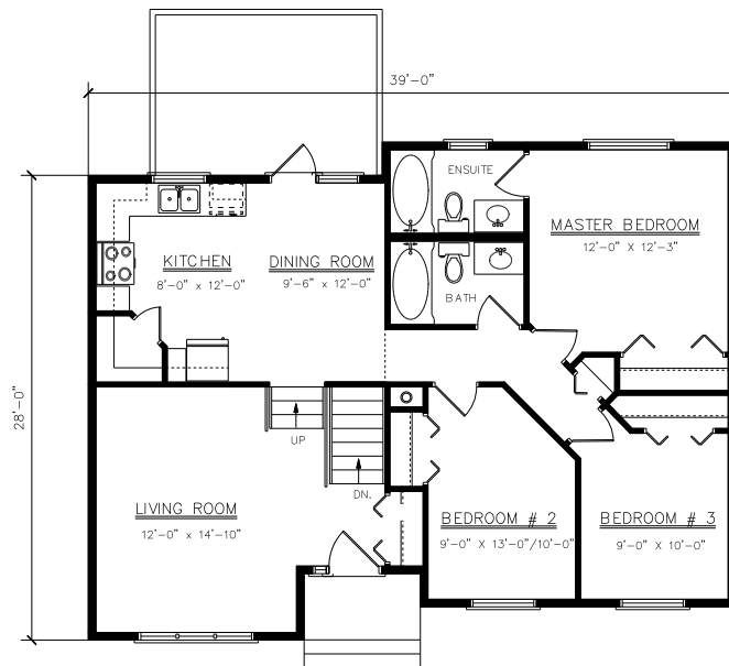
FLOOR PLAN 1068 SQ. FT.
