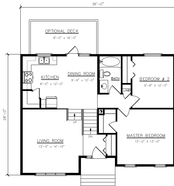
FLOOR PLAN 948 SQ. FT.
