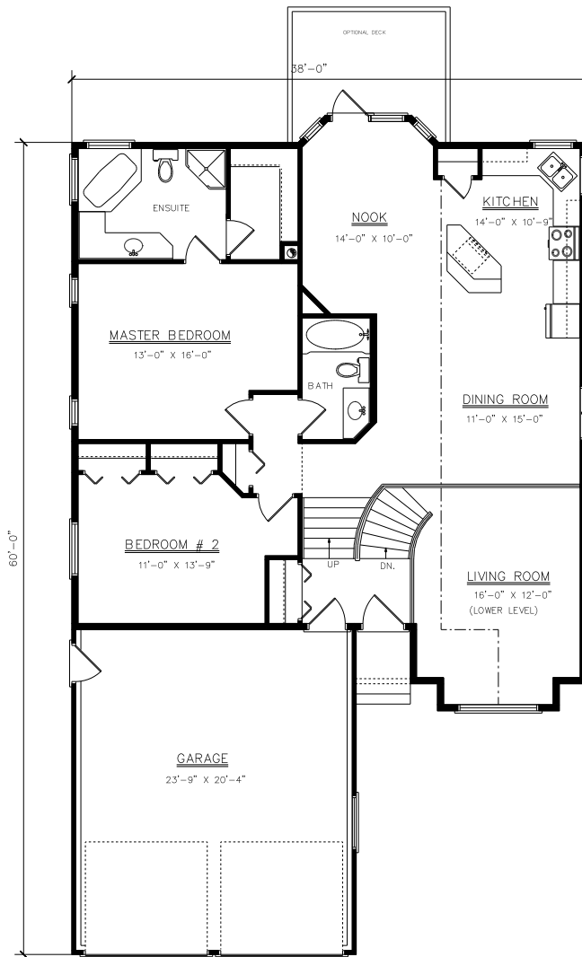
FLOOR PLAN 1454 SQ. FT.
