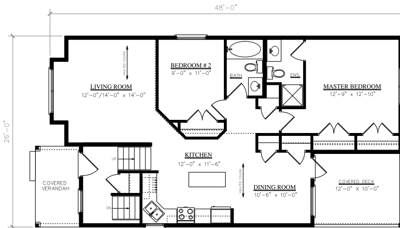
FLOOR PLAN 1072 SQ. FT.
