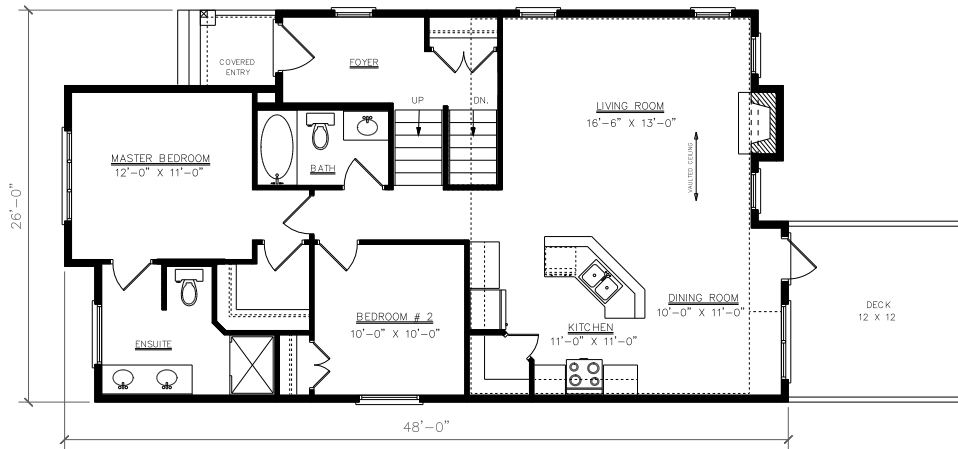
FLOOR PLAN 1132 SQ. FT.
