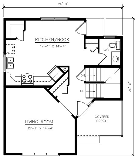
MAIN FLOOR PLAN 636 SQ. FT.
