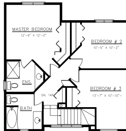
UPPER FLOOR PLAN 750 SQ. FT. 1538 TOTAL SQ. FT.
