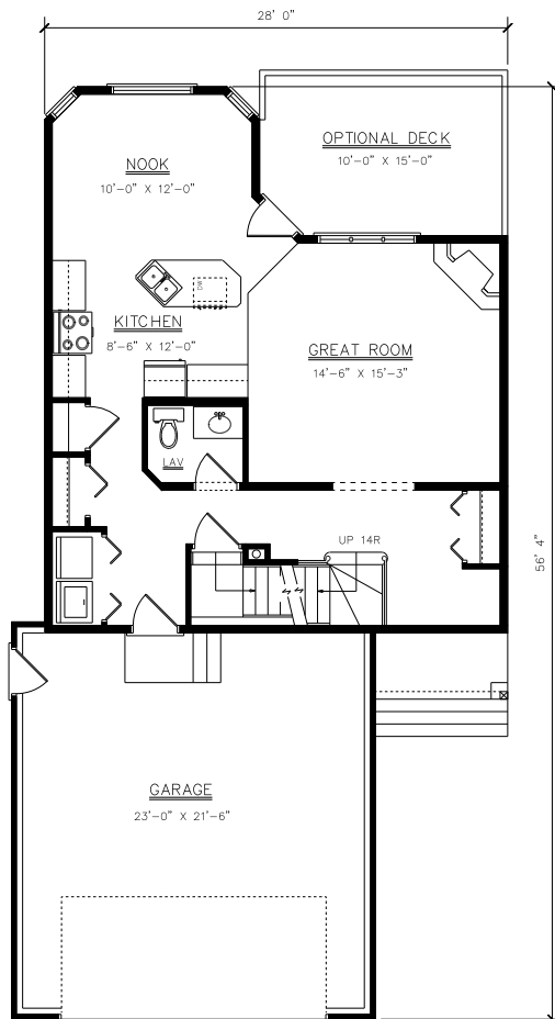
MAIN FLOOR PLAN 788 SQ. FT.
