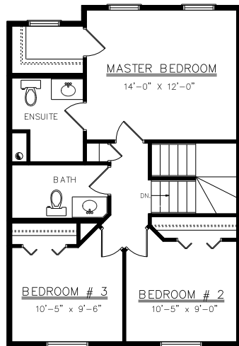
UPPER FLOOR PLAN 694 SQ. FT.
