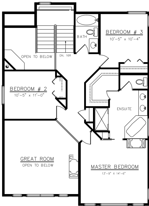
UPPER FLOOR PLAN 876 SQ. FT.
