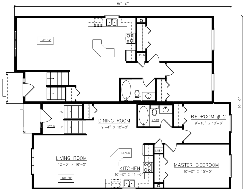
FLOOR PLAN 908 SQ. FT. EACH UNIT 908 SQ. FT.
