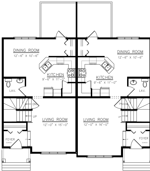
MAIN FLOOR PLAN "A" 670 SQ. FT. 1340 TOTAL SQ. FT.
