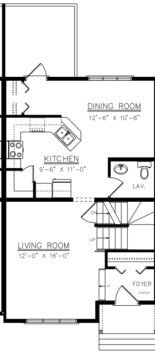
MAIN FLOOR PLAN "B" 683 SQ. FT. 1366 TOTAL SQ. FT.
