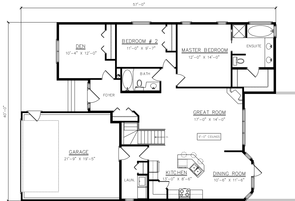
FLOOR PLAN 1488 SQ. FT.
