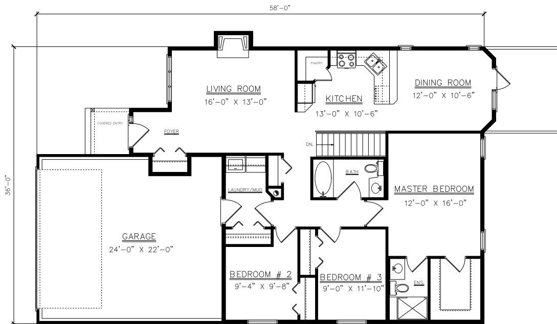
FLOOR PLAN 1384 SQ. FT.
