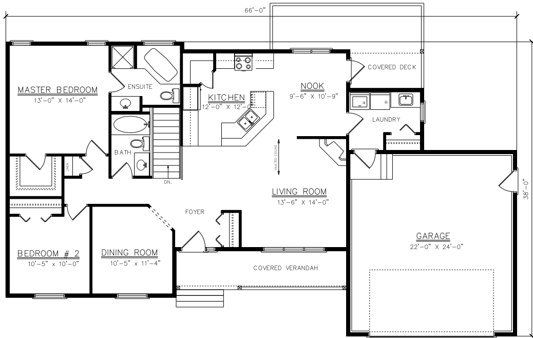
FLOOR PLAN 1392 SQ. FT.
