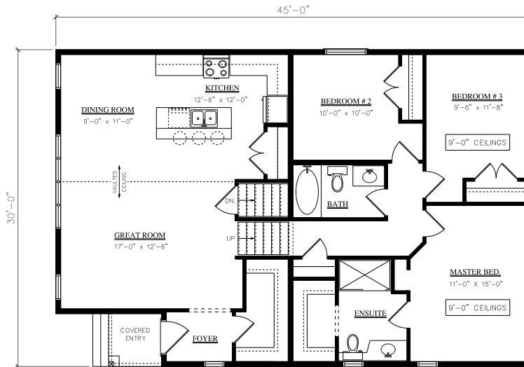
MAIN FLOOR PLAN 1300 SQ. FT.
