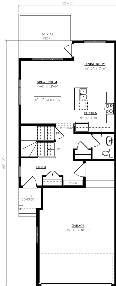
MAIN FLOOR PLAN 636 SQ. FT. 1484 TOTAL SQ. FT.
