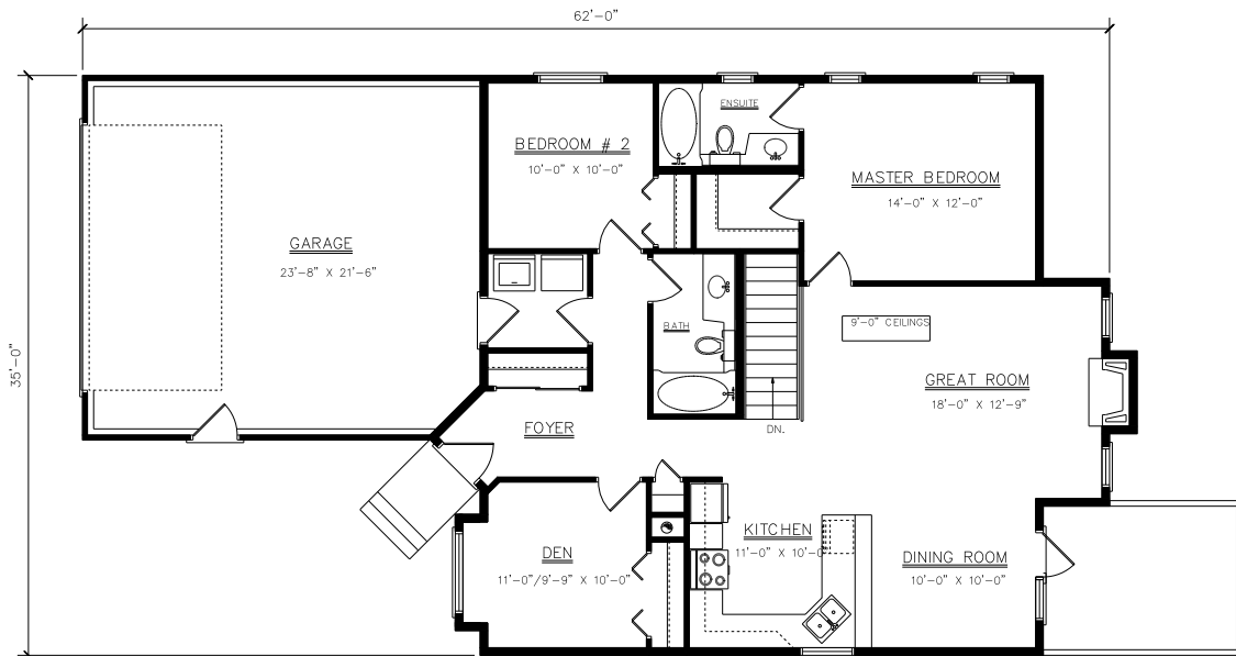
FLOOR PLAN 1266 SQ. FT.
