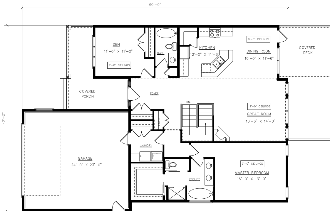
FLOOR PLAN 1512 SQ. FT.
