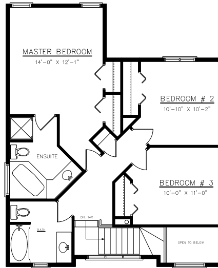
UPPER FLOOR PLAN 836 SQ. FT.
