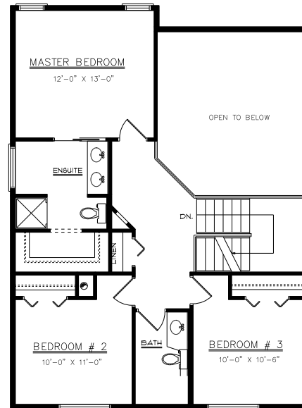
UPPER FLOOR PLAN 820 SQ. FT.
