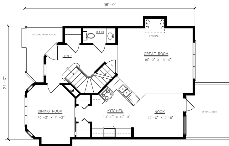
MAIN FLOOR PLAN 785 SQ. FT. 1565 TOTAL SQ. FT.
