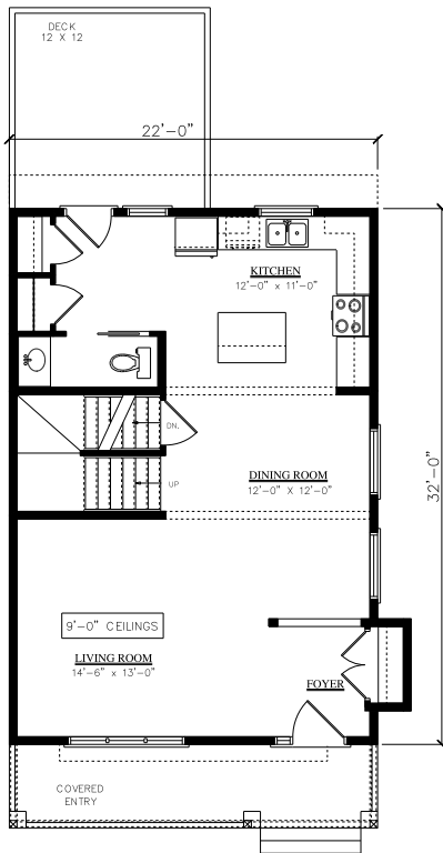
MAIN FLOOR PLAN 715 SQ. FT. 1479 TOTAL SQ. FT.
