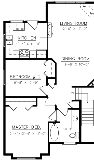
UPPER FLOOR PLAN 877 SQ. FT.
