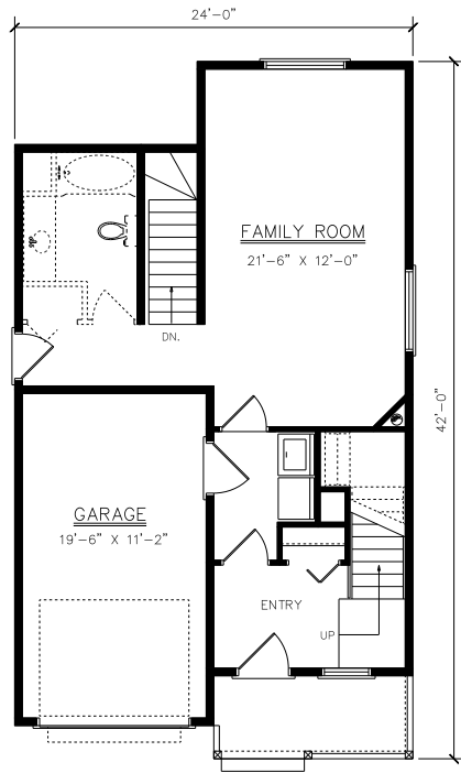
MAIN FLOOR PLAN 637 SQ. FT.
