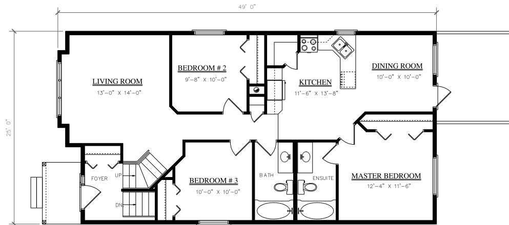
FLOOR PLAN 1190 SQ. FT.
