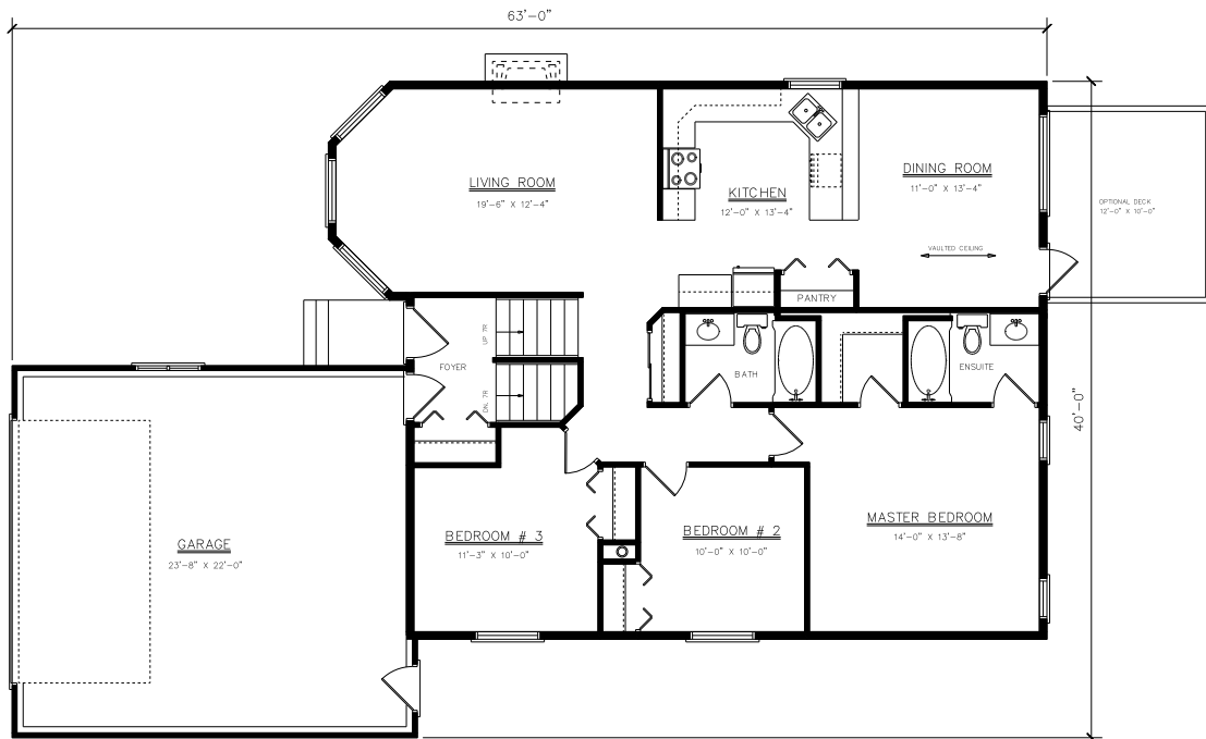
FLOOR PLAN 1375 SQ. FT.
