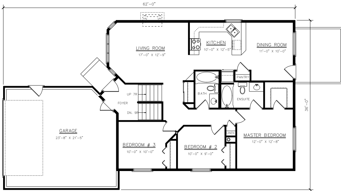
FLOOR PLAN 1248 SQ. FT.
