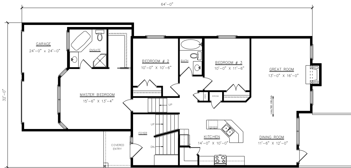
FLOOR PLAN 1472 SQ. FT.
