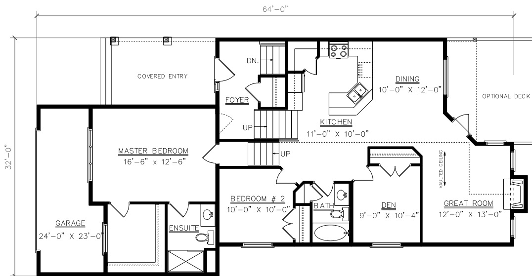
FLOOR PLAN 1376 SQ. FT.
