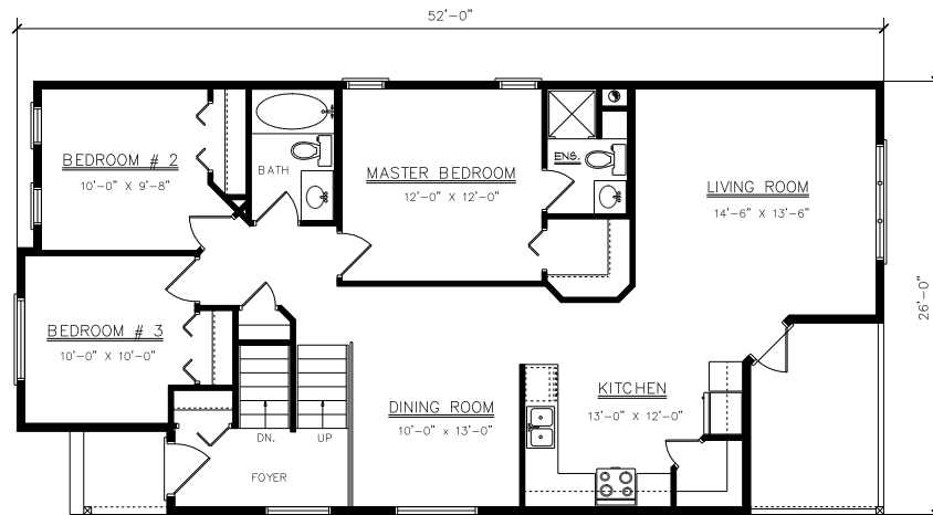
FLOOR PLAN 1208 SQ. FT.
