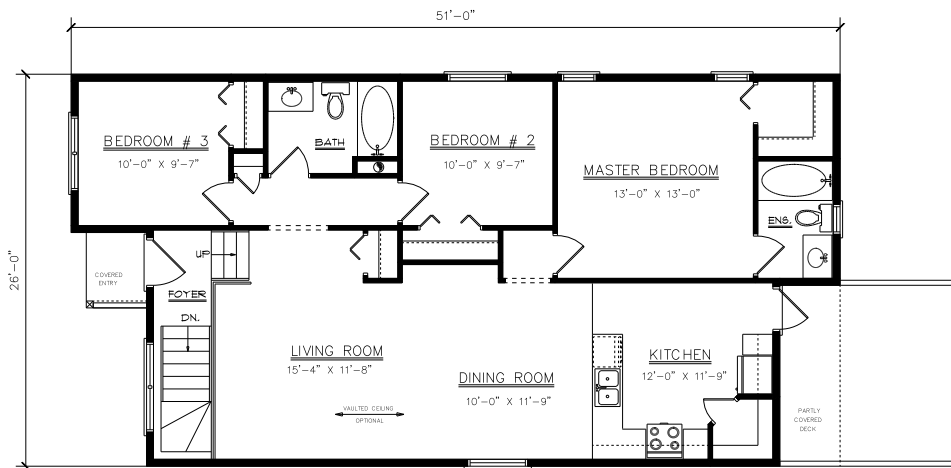
FLOOR PLAN 1201 SQ. FT.
