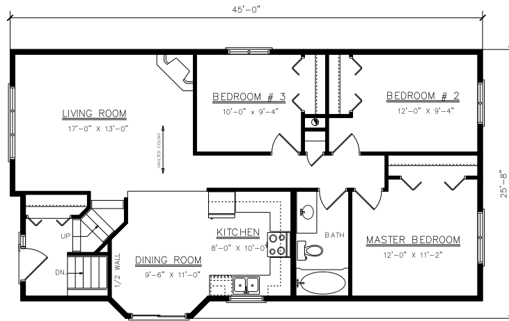
FLOOR PLAN 1082 SQ. FT.
