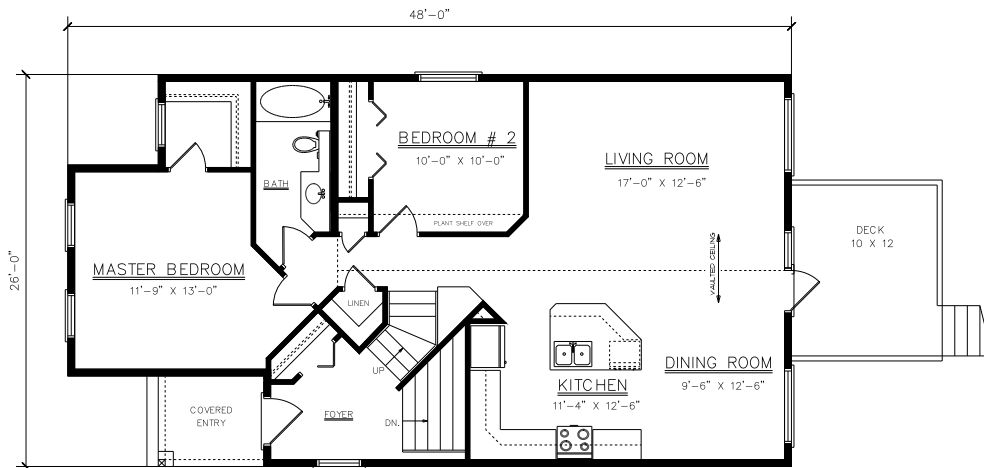
FLOOR PLAN
