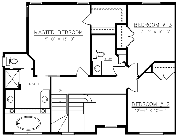
UPPER FLOOR PLAN 848 SQ. FT.
