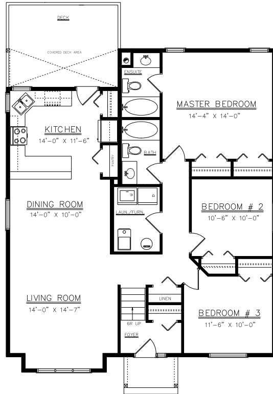
FLOOR PLAN 1456 SQ. FT.
